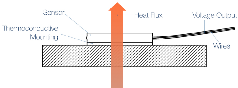
Fig 4.1 Schematic diagram of mounting and functionality of HF03 Heat Flux Sensor.
